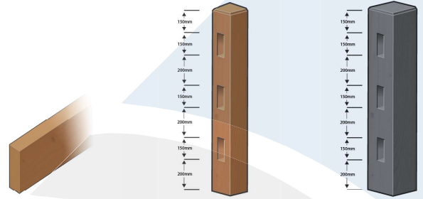
Standard Rail 150x50 Standard Post 150x150 1200 High Optional Post 200x200 1200 High
